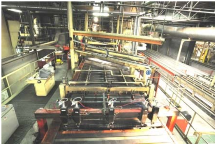
Trimming and sizing saw
